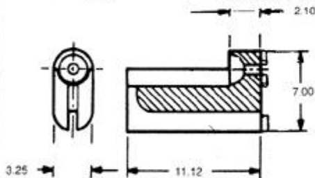
15-3-64 TERMINAL INSULATOR (N)
