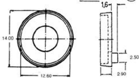
M165 WITH ANTI-ROTATION LUG (P)
